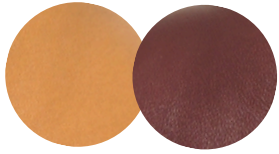
DOFA Camel
